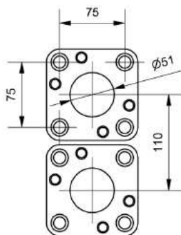
Adapter dimensions SAE 2''-3000M
